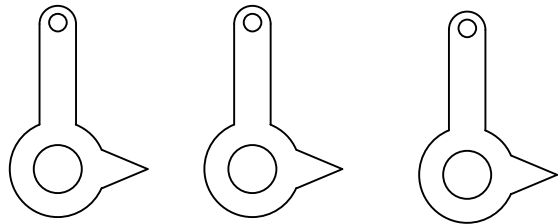
Reversing levers – 3/64" brass sheet
