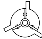
Assemble the unit by pushing the lugs of three plates into the base holes and bending back underneath
