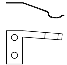
Two types of Meteor/other small motor brush – one dished and the other plain. Made in 7 thou phosphor bronze
