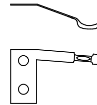
Two types of Meteor/other small motor brush – one dished and the other plain. Made in 7 thou phosphor bronze
